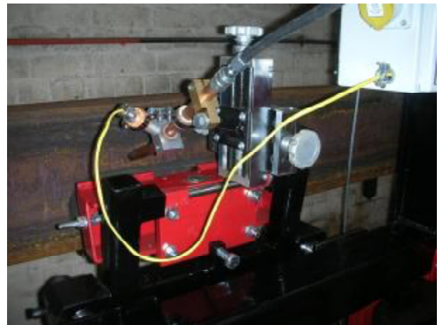
Welding Nozzle Assembly with Flux Transfer & Recovery System, Manual x and y Slides with Laser Guide Light. Set up to weld in the 3 o'clock position.
